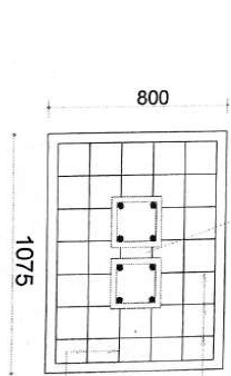
8-10mm \varnothing @150cc along width (Top) 6-10mm \varnothing @150cc along length (Bottom)
