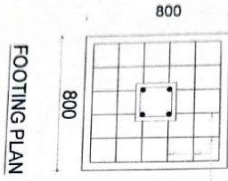
6-10mm \varnothing @150cc both ways
